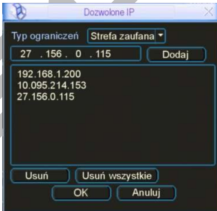
Rys. 5-9a. Dozwolone IP.
