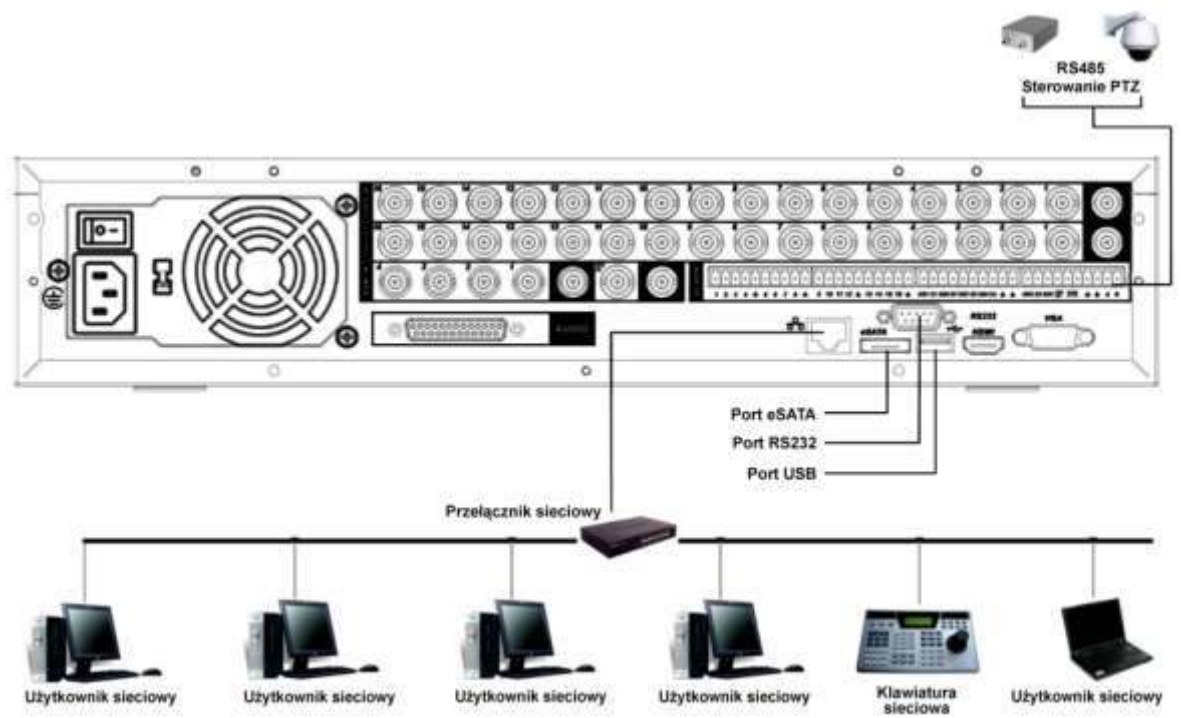
Rys. 3-10. Interfejsy rejestratora: RS232, RS485, USB, LAN
